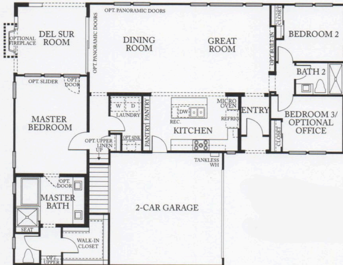
FIRST STORY
