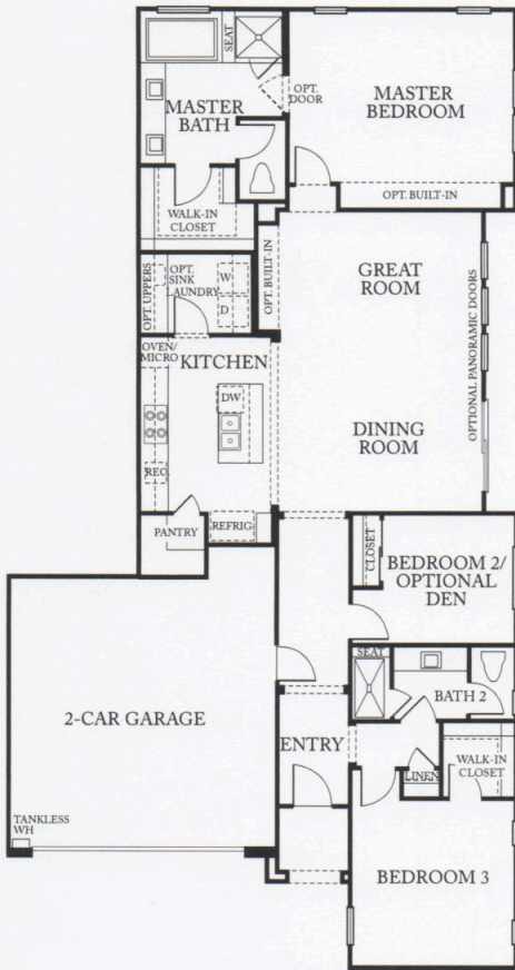
OPTIONAL EXPANDED SHOWER AT MASTER BATH
