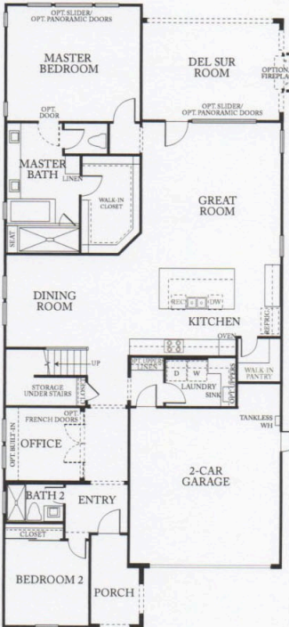
FIRST STORY
