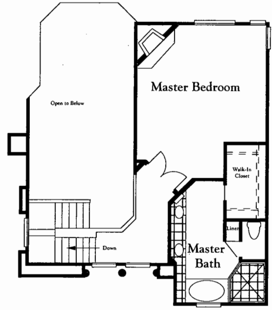
Madeira Second Floor
