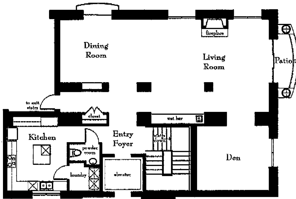
Second Level
