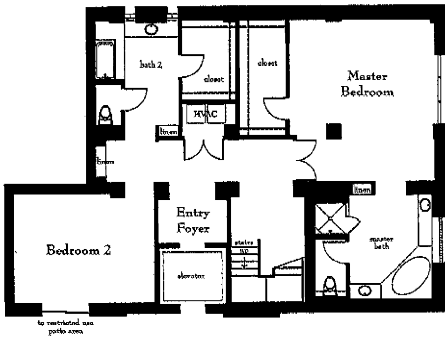
First Level
