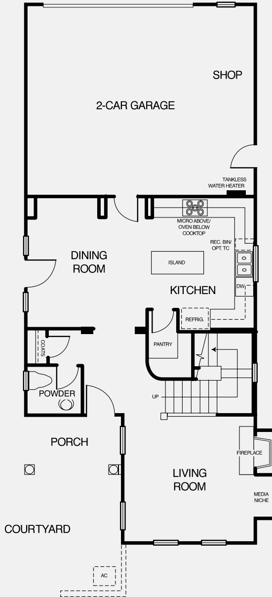
PLAN 3B FIRST STORY
