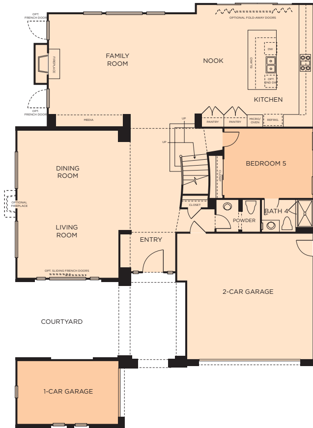
FIRST STORY
