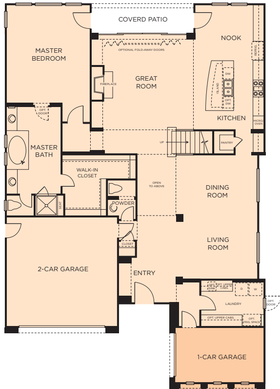
FIRST STORY
