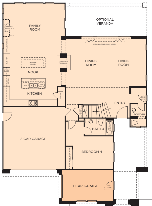
FIRST STORY
