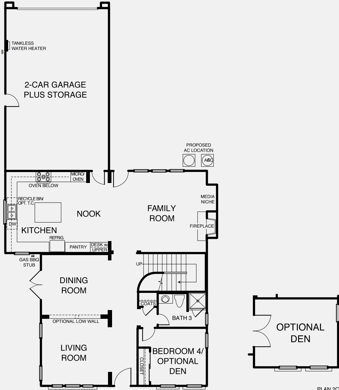
PLAN 2C FIRST STORY
