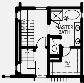
STAIRS AT BONUS OPTION
