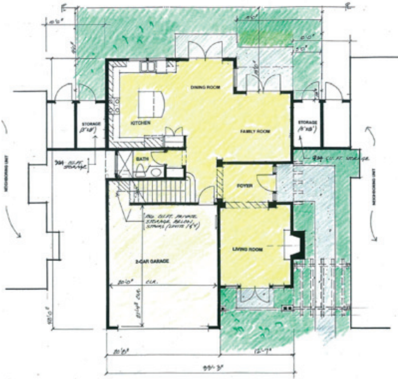
1 ST FLOOR PLAN UNITS 2, 3, & 4
