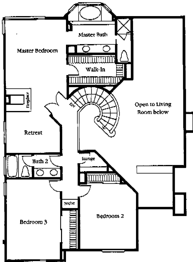
Second Floor
