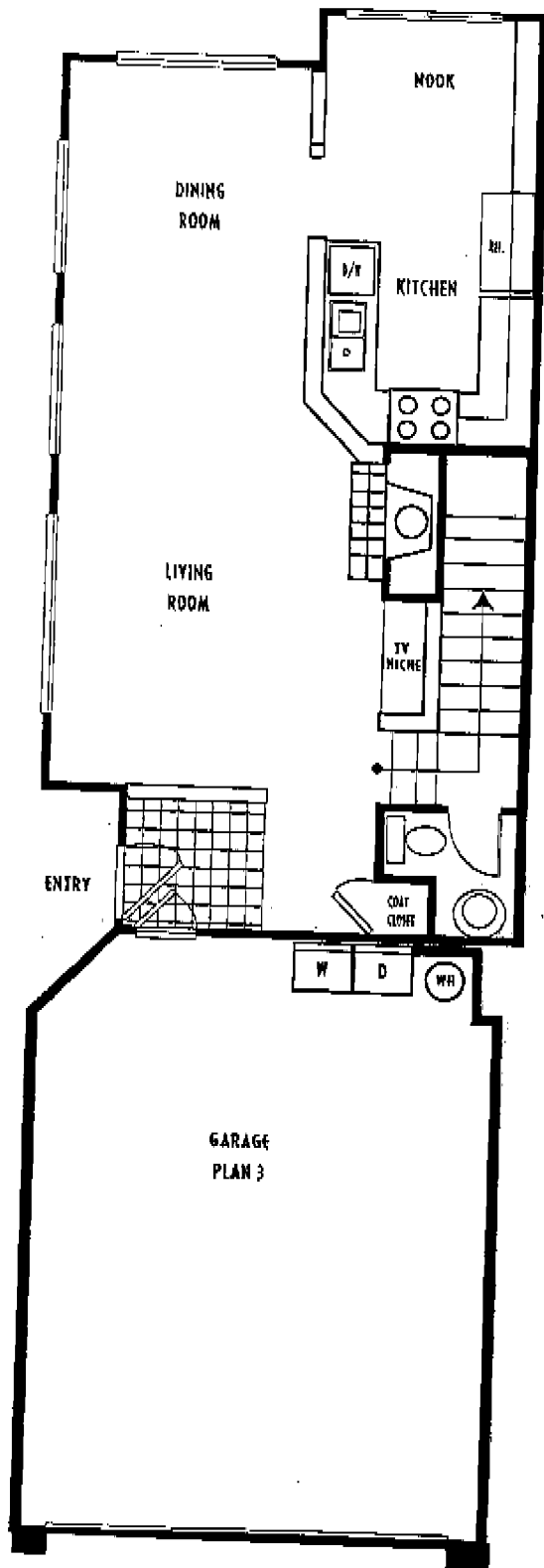
FIRST FLOOR
