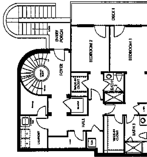
LOWER FLOOR
